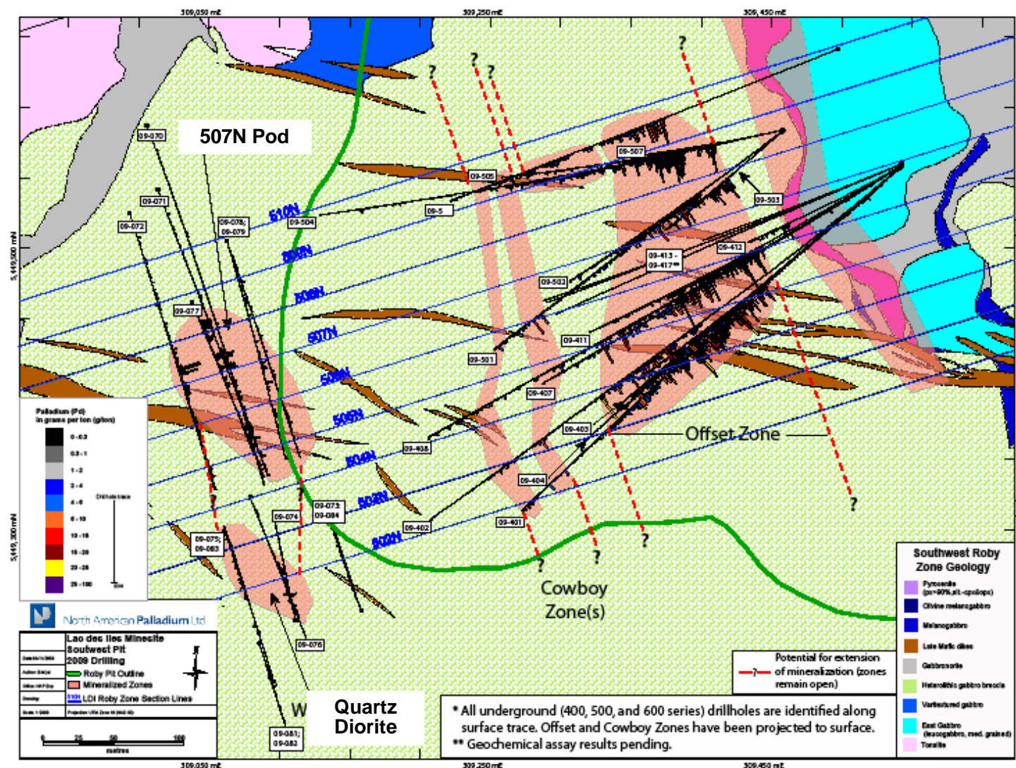
Figure 5. Phases 1 and 2 drilling in the West Pit area of the Lac des Iles mine.
