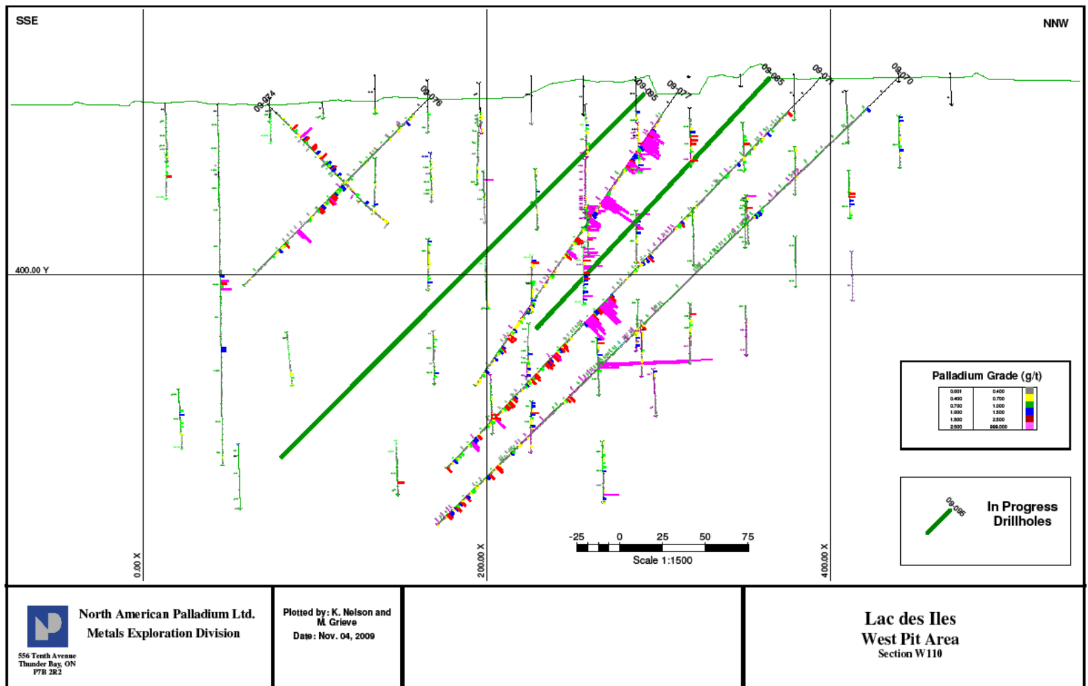
Figure 6. Cross section W110 of the West Pit area showing the 2009 drill traces and assay results for palladium.
